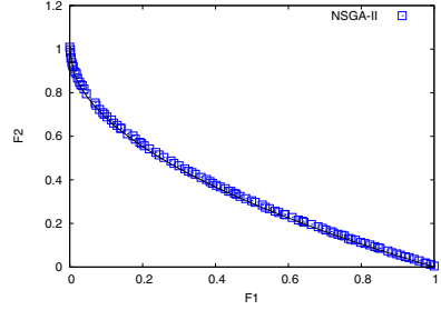
Fig. 5.2 Results of ZDT1 obtained by NSGA-II using 10,000 function evaluations
