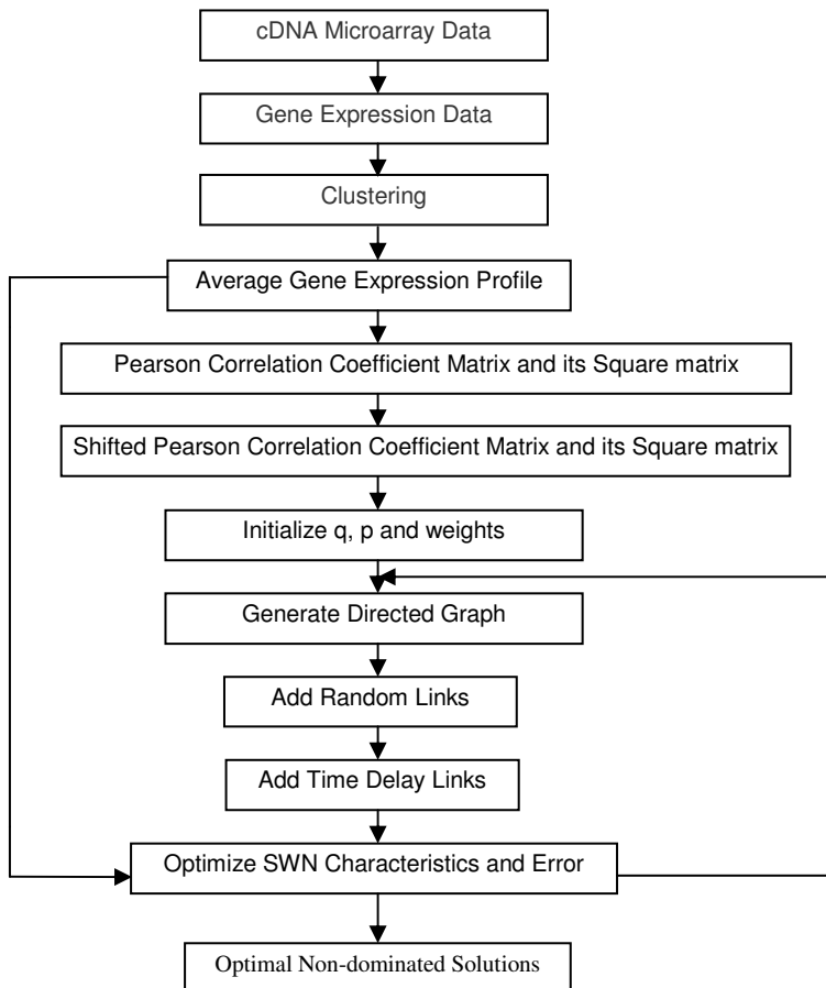
Fig. 12.1 A schematic flowchart of the overall algorithm
