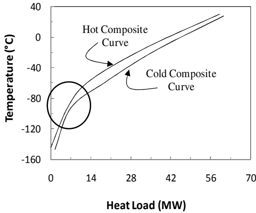
Fig. 8.20 Composite curves for the Pareto-optimal solution corresponding to the lowest shaftwork and the highest capital cost in Fig. 8.18: C_{total} = \$ 12.9 Million, W_{total} = 28.29 MW, \Delta T_{min} = 2.73 °C, n_{NG} = 3 , n_{N2} = 1 , A_{total} = 92574 m 2 .
