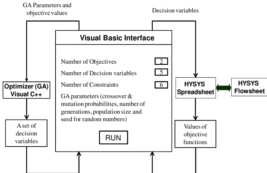
Fig. 8.8 Architecture and working principle of MPMLE.
