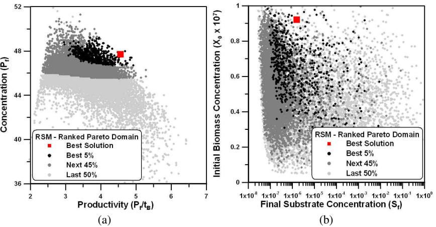
Fig. 7.16 Ranked Pareto domain for the four-objective optimization of gluconic acid using RSM with relative weights: (a) concentration versus productivity of gluconic acid; (b) initial biomass concentration versus final substrate concentration.
