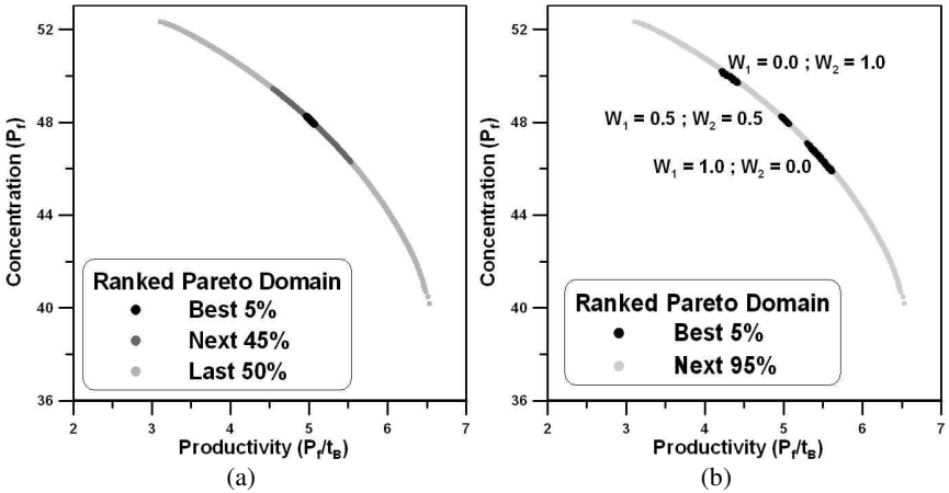
Fig. 7.4 Ranked Pareto domain using NFM for the two-objective optimization of gluconic acid: (a) Nominal case; (b) Influence of the relative weights of the two objective functions.
