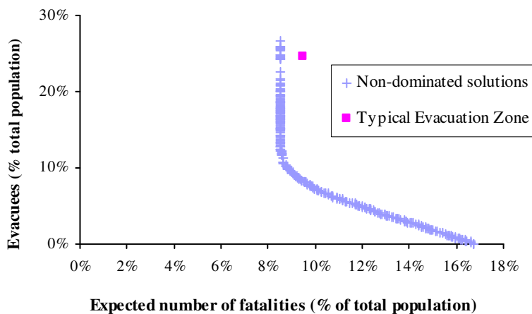
Fig. 11.7 Non-dominated solutions (ERPs) in case of a BLEVE phenomenon in an LPG storage tank (“capacity” of the transportation network: 1, “warning time”: 3600 sec).
