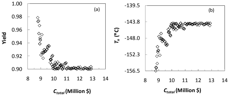
Fig. 8.22 Values of constraints corresponding to the Pareto-optimal solutions shown in Figs. 8.18 and 8.21: (a) yield of LNG; and (b) final refrigeration temperature, T_n .
