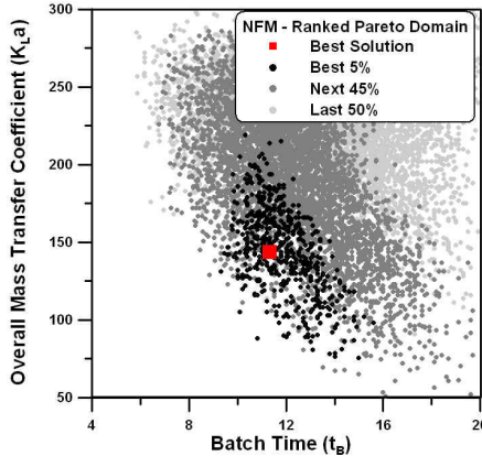
Fig. 7.9 Plot of the input space for the four-objective Pareto domain: K_La versus t_B .
