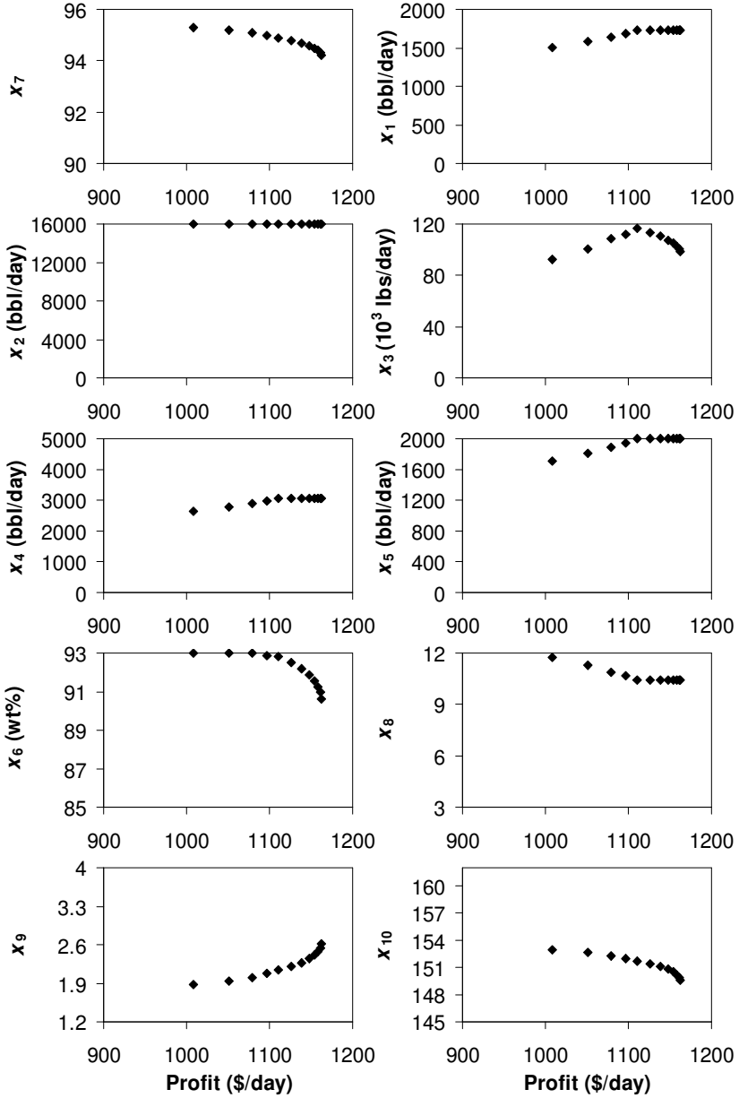
Fig. 1.5 Pareto-optimal solutions for maximizing profit and octane number ( x_7 ) by the \varepsilon -constraint method; profit is shown on the x-axis in all plots.
