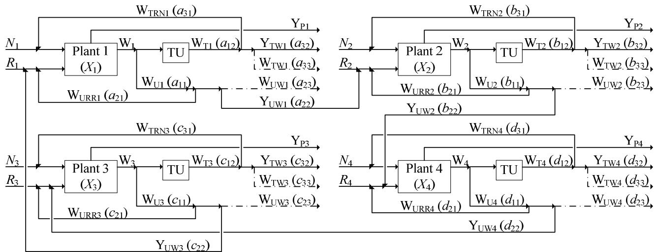
Fig. E.3 An IE system with 4 plants for exercise 10.3.
