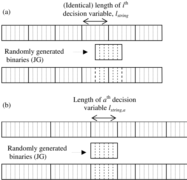
Fig. 4.7 The (a) saJG and (b) sJG operations
