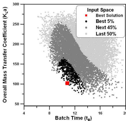
Fig. 7.7 Plot of the input space for the three-objective optimization problem associated with the Pareto domain: K_L a versus t_B .
