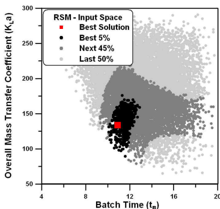
Fig. 7.15 Plot of the input space for the three-objective Pareto domain using RSM with relative weights: K_{La} versus t_B .
