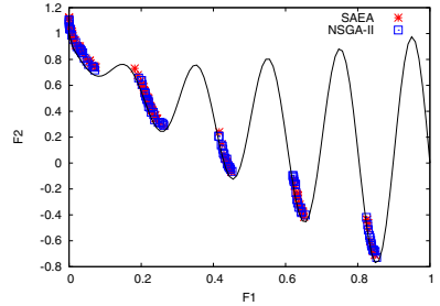
Fig. 5.4 Results of ZDT3 obtained by SAEA and NSGA-II using limited number of function evaluations
