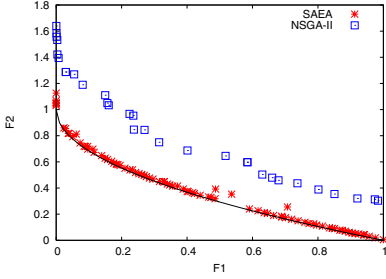
Fig. 5.1 Results for ZDT1 obtained by SAEA and NSGA-II using limited number of function evaluations
