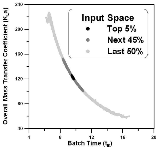
Fig. 7.5 Plot of the input space for the two-objective optimization problem associated with the Pareto domain: K_La versus t_B .
