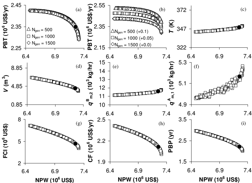
Fig. 10.3 Optimal results of the WO process for multiple objectives – Case A; for clarity, results in (a) are re-plotted in (b) with suitable vertical shifts in the ordinate; NPW is shown on the x-axis in all plots.
