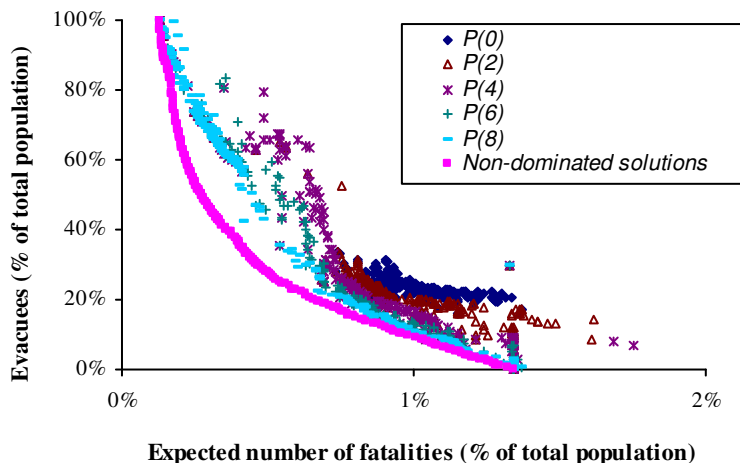
Fig. 11.5 Evolution of “population” of emergency response plans.
