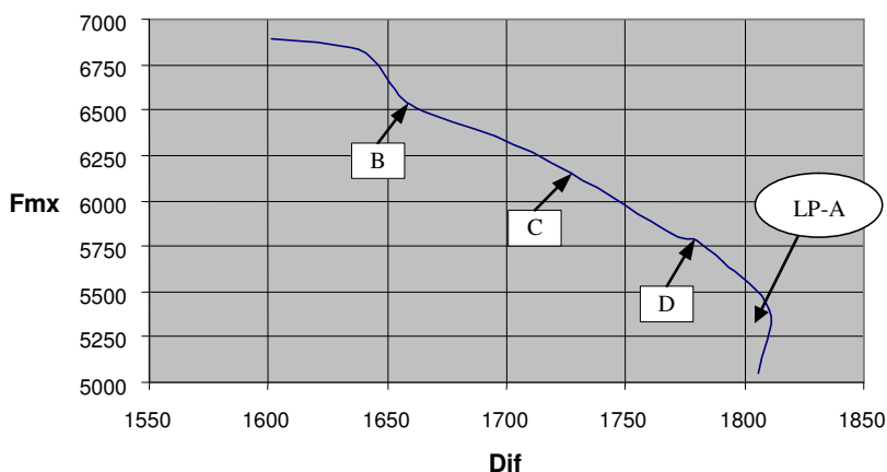
Fig. 9.5 Conflicting Objectives: F_{mx} Versus Dif .
