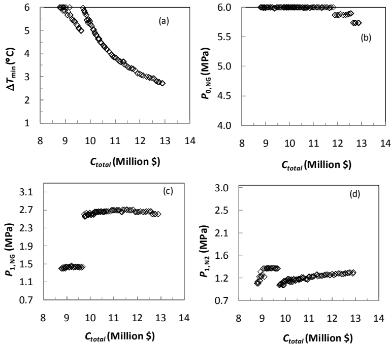
Fig. 8.21 Values of decision variables corresponding to the Pareto-optimal front in Fig. 8.17: (a) heat exchanger \Delta T_{min} ; (b) initial refrigerant pressure in the natural gas loop, P_{0,NG} ; (c) final natural gas refrigerant pressure, P_{1,NG} ; and (d) final N_2 refrigerant pressure, P_{1,N_2} .
