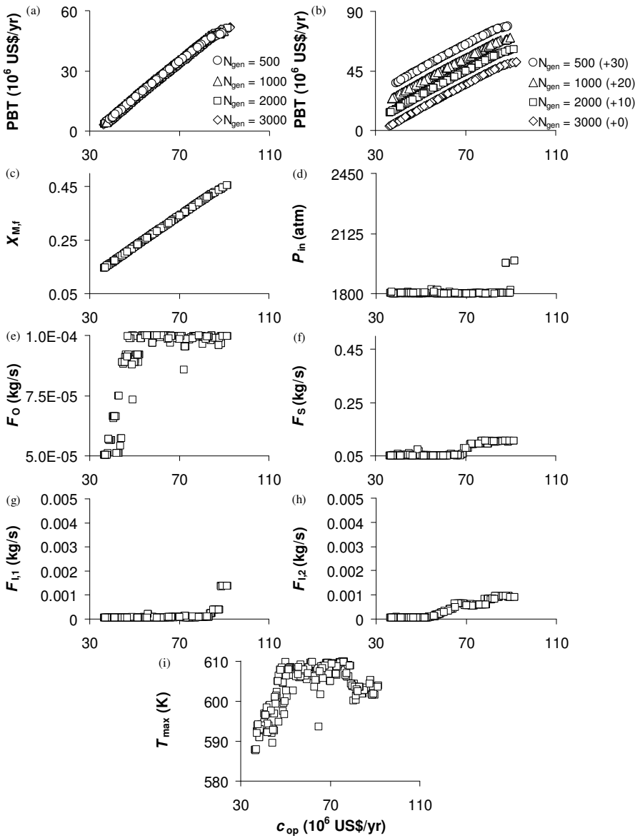
Fig. 10.6 Optimization of LDPE plant by NSGA-II-aJG – Case C; for clarity, results in (a) are re-plotted in (b) with suitable vertical shifts in the ordinate; c_{op} is shown on the x-axis in all plots.
