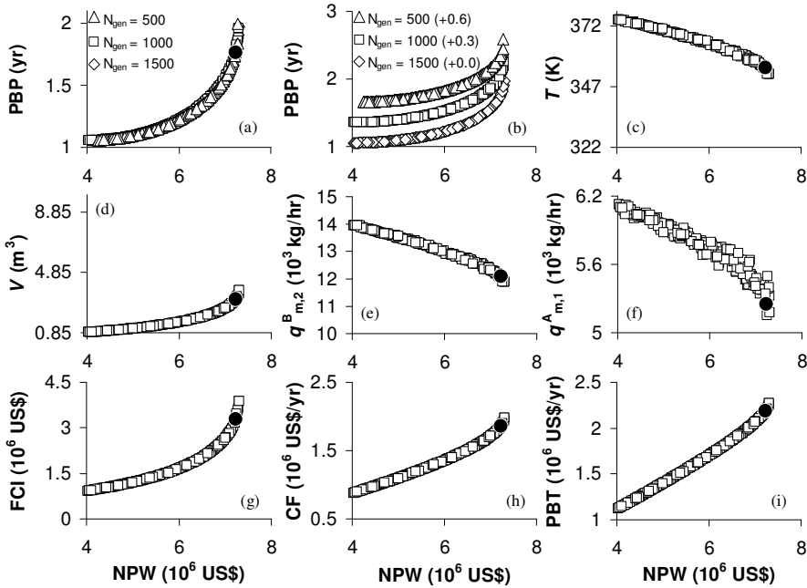
Fig. 10.4 Optimal Results of WO Process for Multiple Objectives – Case B; for clarity, results in (a) are re-plotted in (b) with suitable vertical shifts in the ordinate; NPW is shown on the x-axis in all plots.
