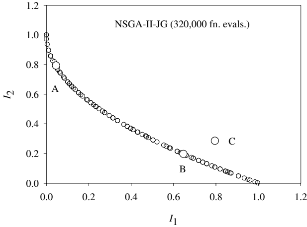
Fig. 4.1 The Pareto set obtained for the ZDT4 problem (Deb, 2001) using NSGA-II-JG. An additional point, C, is also indicated
