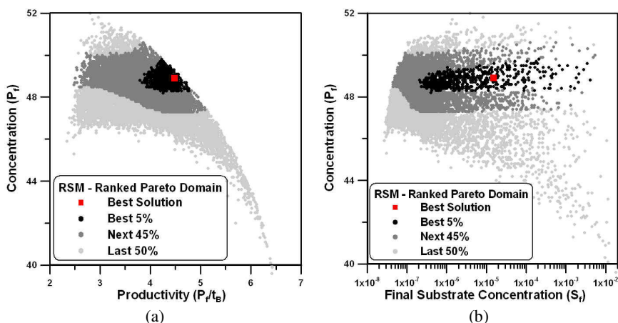
Fig. 7.14 Ranked Pareto domain for the three-objective optimization of gluconic acid using RSM with relative weights: (a) concentration versus productivity of gluconic acid; (b) gluconic acid concentration versus the final substrate concentration.
