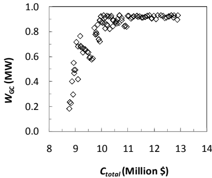
Fig. 8.23 Amount of shaftwork required in the fuel gas compressor corresponding to the Pareto-optimal solutions shown in Fig. 8.18.
