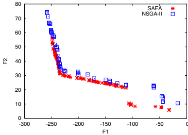
Fig. 5.5 Results of OSY obtained by SAEA and NSGA-II using limited number of function evaluations
