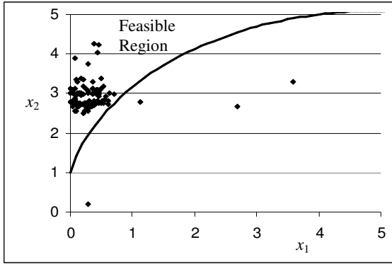
Fig. 4.4 Population at the 40 th generation for the constrained optimization problem in Eq. 4.8
