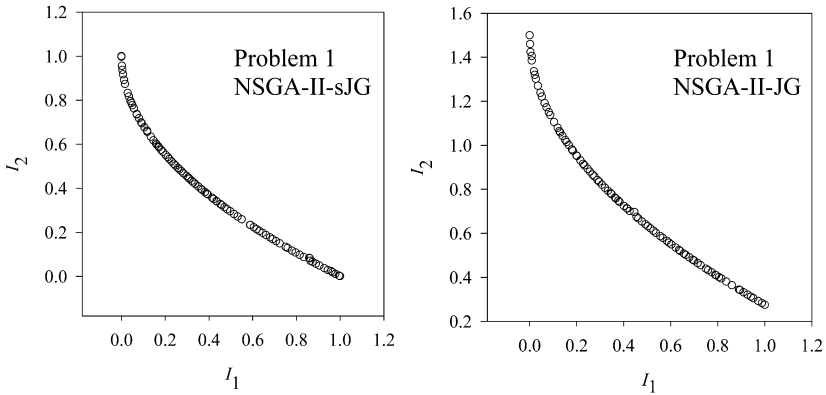
Fig. 4.9 Optimal solutions for the ZDT4 problem after 1,000 generations (200,000 function evaluations) using NSGA-II-sJG and NSGA-II-JG (Agarwal and Gupta, 2007a)
