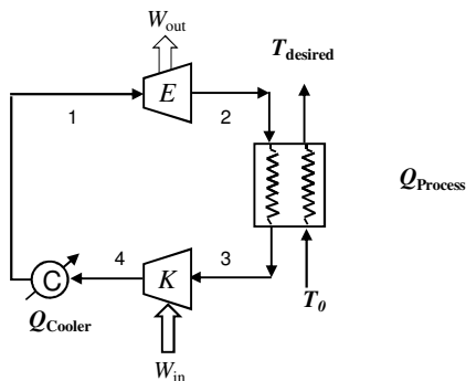
Fig. 8.E1 A single stage gas-phase refrigeration process.
