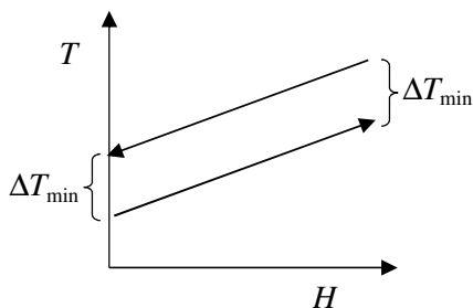
Fig. 8.7 Composite curves of a heat exchange process showing \Delta T_{\min} .
