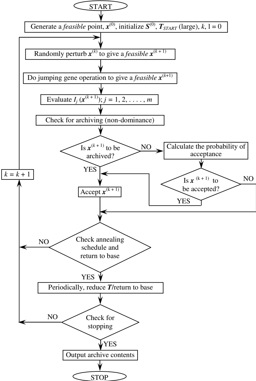
Fig. 4.A 1 Flowchart for MOSA-JG/aJG
