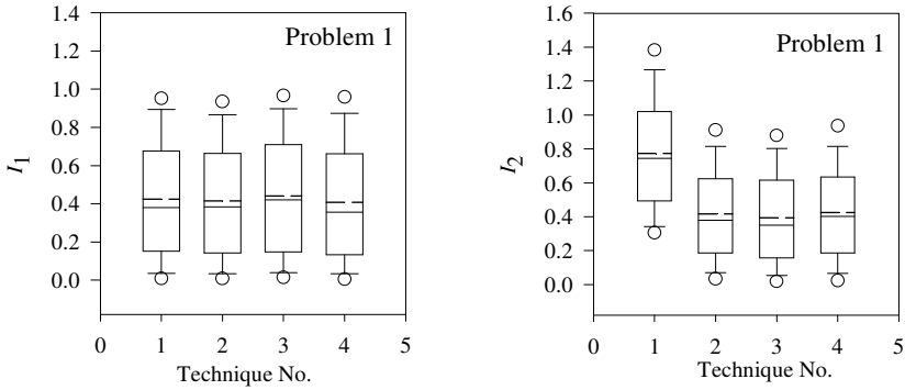
Fig. 4.10 Box plots of I_1 and I_2 for the ZDT4 problem after 1,000 generations; Technique 1: NSGA-II-JG; 2: NSGA-II-aJG; 3: NSGA-II-saJG; 4: NSGA-II-sJG (Agarwal and Gupta, 2007a)
