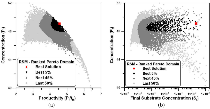
Fig. 7.12 Ranked Pareto domain for the three-objective optimization of gluconic acid using RSM without rules (011) and (100): (a) concentration versus productivity of gluconic acid; (b) gluconic acid concentration versus final substrate concentration.
