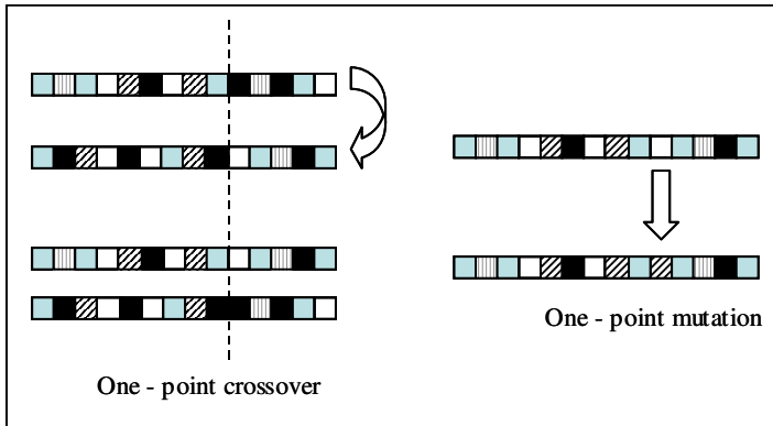
Fig. 11.4 Examples of one-point crossover and one-point mutation.
