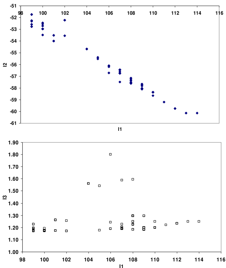
Fig. 12.5(a) Non-dominated Pareto solutions
