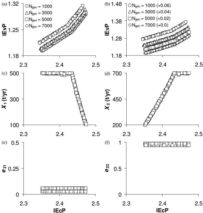
Fig. 10.8 MOO of the IE with 6 plants for maximizing IEcP and minimizing IEvP; for clarity, results in (a) are re-plotted in (b) with suitable vertical shifts; IEcP is shown on the x-axis in all plots.
