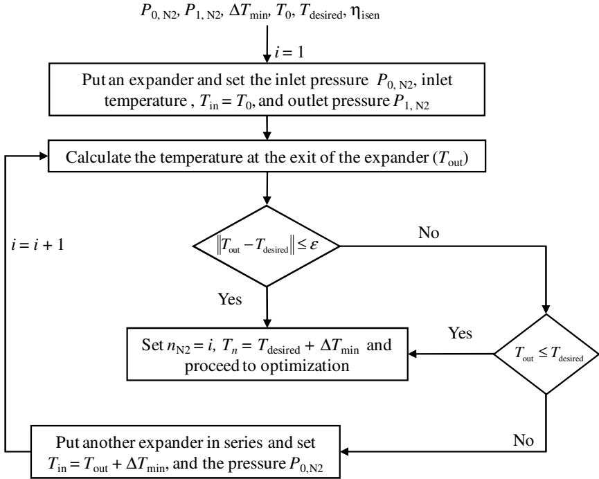
Fig. 8.11 Algorithm to calculate the number of refrigeration stages.
