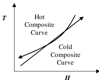
Fig. 8.10 Composite curves showing internal pinching in a heat exchanger.
