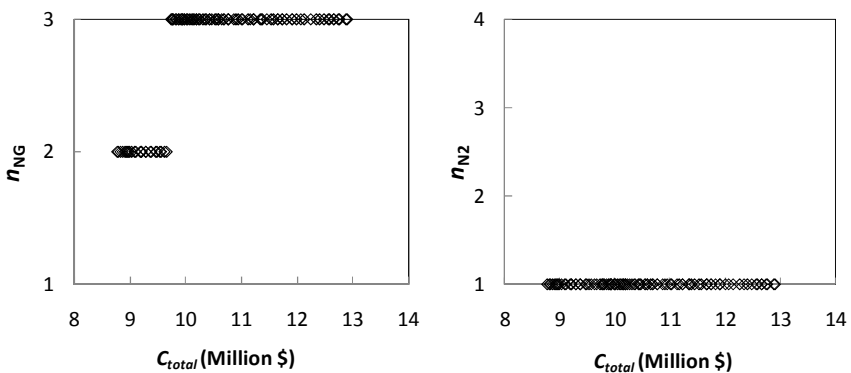
Fig. 8.19 Number of natural gas and number of nitrogen refrigeration stages corresponding to the Pareto-optimal front in Fig. 8.18.
