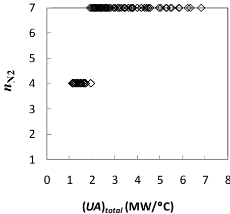
Fig. 8.13 Number of stages corresponding to the Pareto-optimal front in Fig. 8.12.
