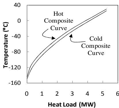
Fig. 8.15 Composite curves for one Pareto-optimal solution corresponding to the minimum UA = 1.12 MW/°C in Fig. 8.12.
