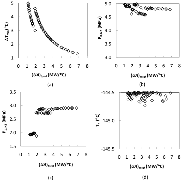
Fig. 8.14 Values of the decision variables and constraint corresponding to the Pareto-optimal front in Fig. 8.12: (a) heat exchanger \Delta T_{min} ; (b) initial refrigerant pressure, P_{0,N2} ; (c) final refrigerant pressure, P_{1,N2} ; and (d) final product temperature, T_n .
