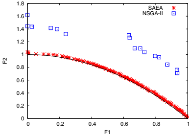
Fig. 5.3 Results of ZDT2 obtained by SAEA and NSGA-II using limited number of function evaluations
