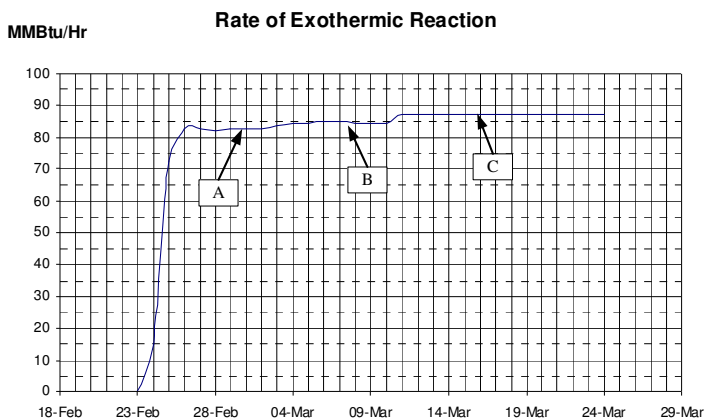
Fig. 9.10 The Exothermic Reaction Rate of Reactor 72CC.
