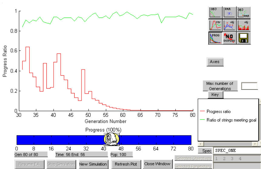
Fig. 9.4 Progressive ratio along the evolution.
