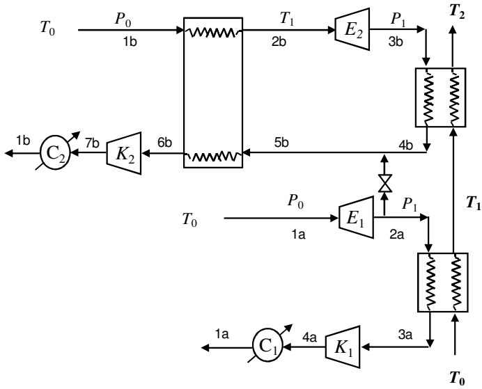
Fig. 8.E2 A two-stage gas-phase refrigeration process.
