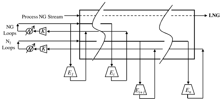
Fig. 8.6 Schematic of the dual independent expander refrigeration process.
