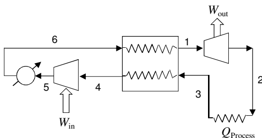
Fig. 8.3 Reverse-Brayton refrigeration cycle.
