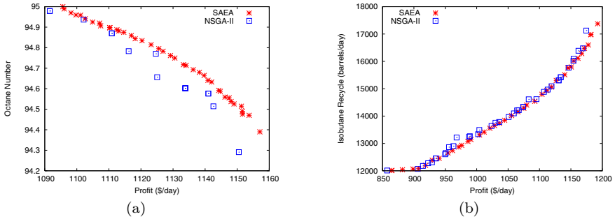
Fig. 5.7 Results obtained by SAEA and NSGA-II for alkylation process optimization. (a) Case A. (b) Case B.
