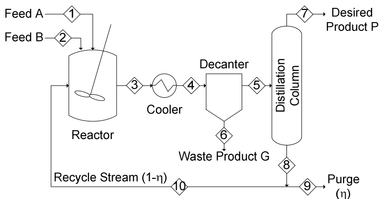
Fig. 10.1 Schematic of the WO Process with stream numbers used in the model.
