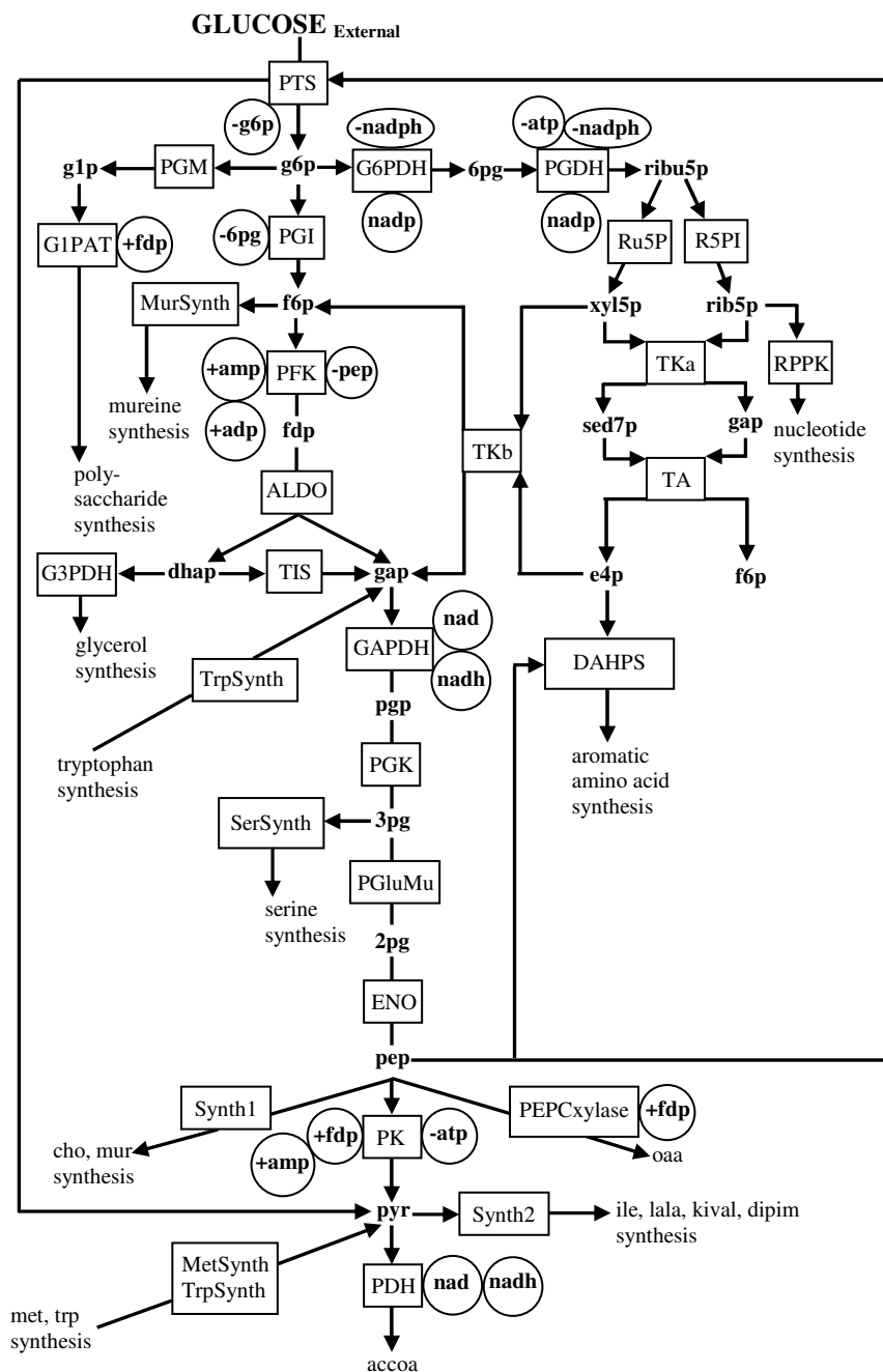
Fig. 13.1 Central carbon metabolism of Escherichia coli . See Section 13.2 for details.
