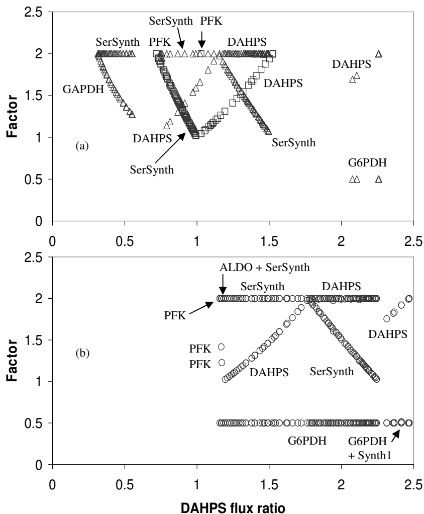
Fig. 13.4B Pareto-optimal enzyme manipulation factors in simultaneous maximization of DAHPS and SerSynth flux ratios (case B) (a) 1-enzyme (□) and 2-enzyme (Δ) manipulation and (b) 3-enzyme manipulation (○).
