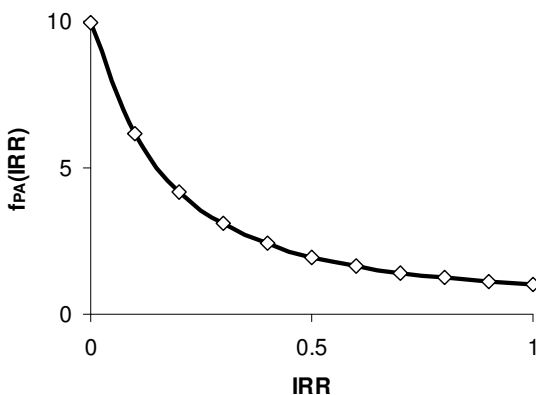
Fig. 10.2 Variation of f_{PA}(\text{IRR}) (= PBP) with IRR.
