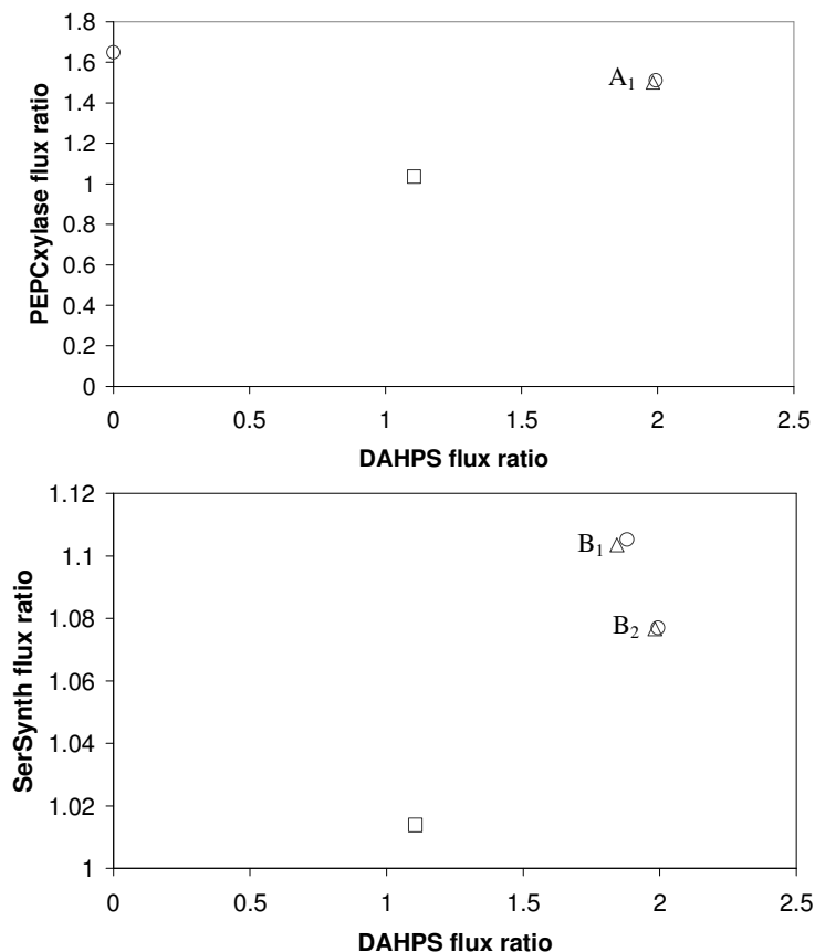
Fig. 13.2 Pareto results for gene knockouts (single-gene \square ; double-gene \Delta ; triple-gene \circ ) in simultaneous maximization of (a) DAHPS and PEPCxylase flux ratios, and (b) DAHPS and SerSynth flux ratios. The chromosomes in double-gene knockouts are labelled.
