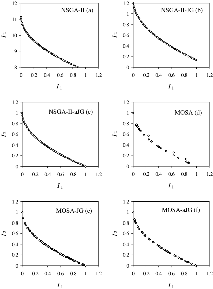
Fig. 4.11 Comparison of the optimal solutions of the ZDT4 problem obtained by different algorithms after 80,000 function evaluations (adapted from Sankararao, 2007)
