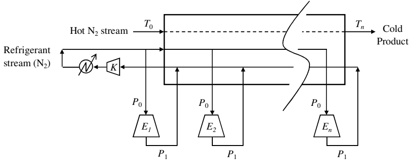
Fig. 8.9 Process flow diagram for nitrogen cooling with nitrogen gas as the refrigerant.
