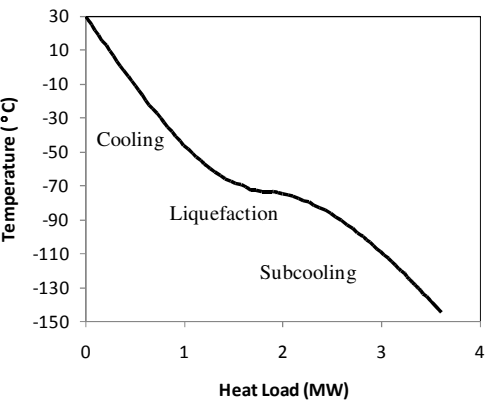
Fig. 8.5 Grand composite curve for LNG.
