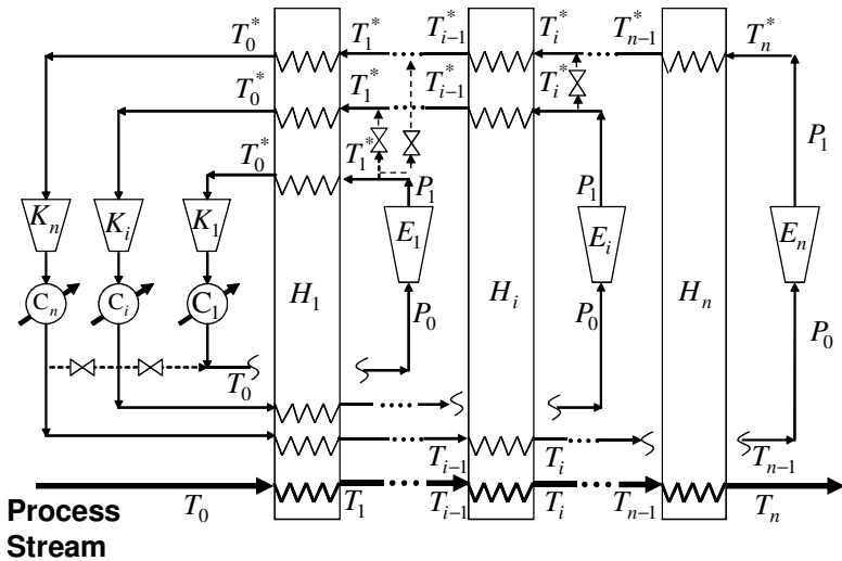
Fig. 8.4 A theoretical multi-stage refrigeration process.
