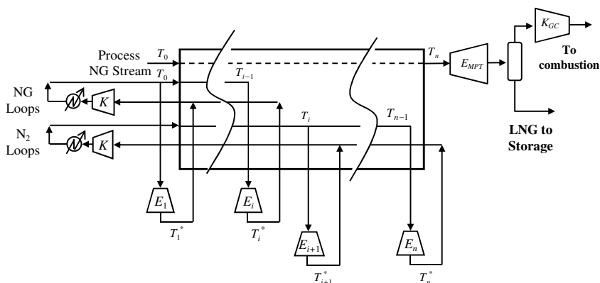
Fig. 8.16 Schematic of the dual independent expander refrigeration process.
