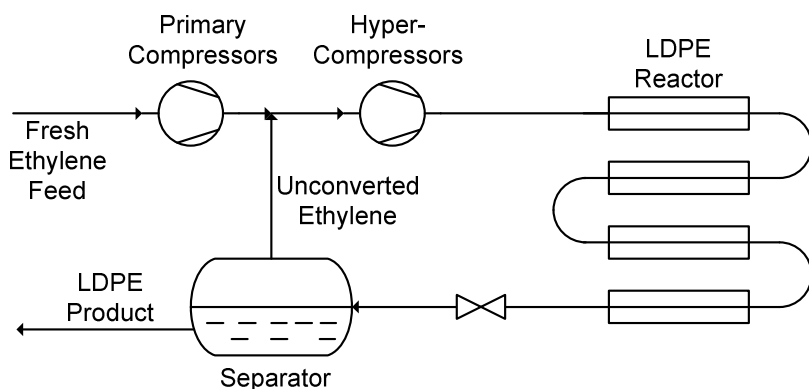
Fig. 10.5 Simplified schematic of an LDPE plant.
