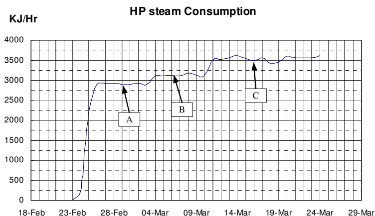
Fig. 9.9 HP Steam Consumption of Reactor 72CC.
