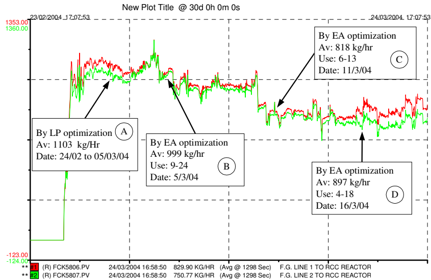
Fig. 9.8 The Fuel Gas Consumption of Reactor 72CC.
