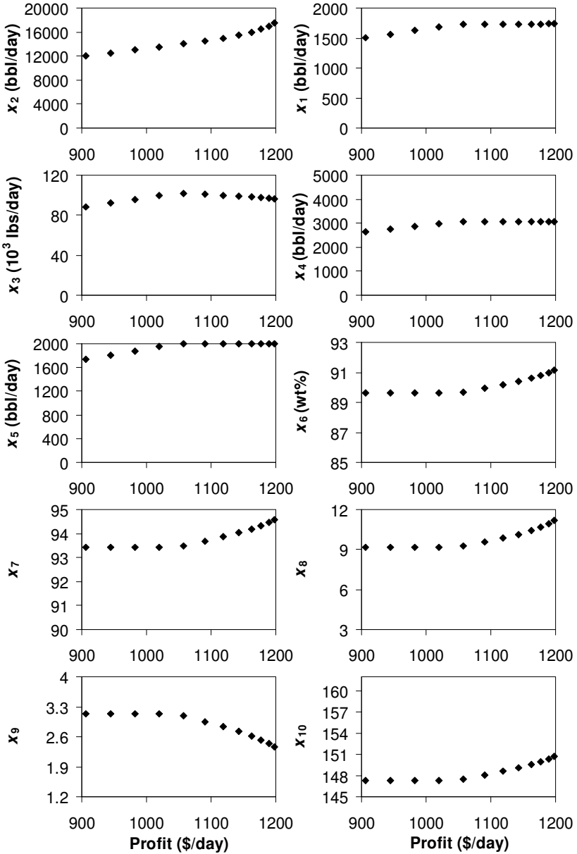
Fig. 1.6 Pareto-optimal solutions for maximizing profit and isobutane recycle ( x_2 ) by the \varepsilon -constraint method; profit is shown on the x-axis in all plots.
