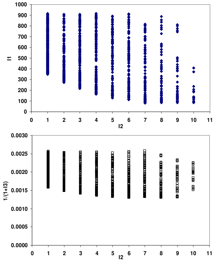
Fig. 12.3(b) Pareto optimal solutions
