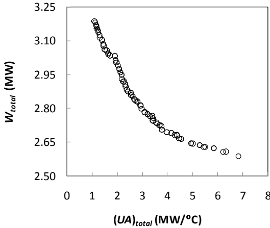
Fig. 8.12 Pareto-optimal front for nitrogen cooling process.
