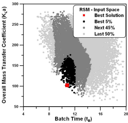
Fig. 7.13 Plot of the input space for the four-objective Pareto domain using RSM without rules (011) and (100): K_L a versus t_B .
