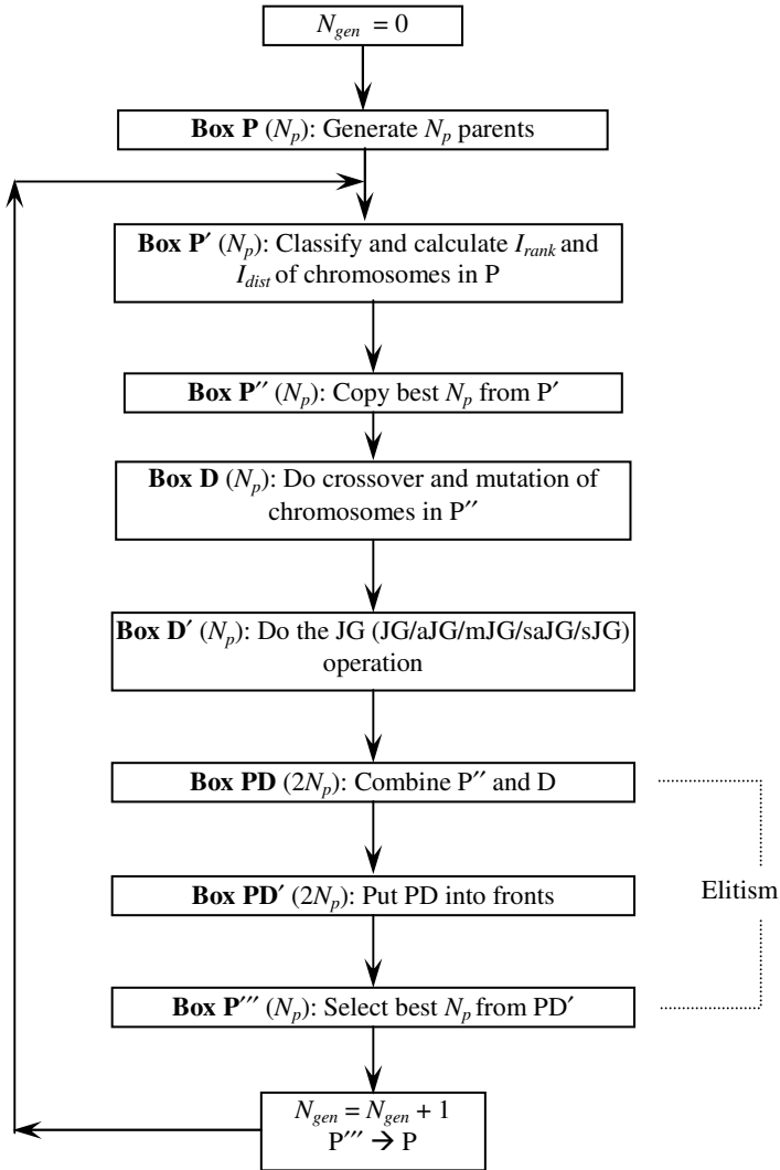
Fig. 4.5 Flowchart for NSGA-II-JG/aJG/mJG/saJG/sJG
