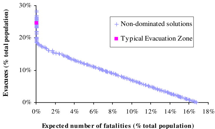
Fig. 11.8 Non-dominated solutions (ERPs) in case of a BLEVE phenomenon in an LPG storage tank (“capacity” of the transportation network: 5, “warning time”: 1800 sec).
