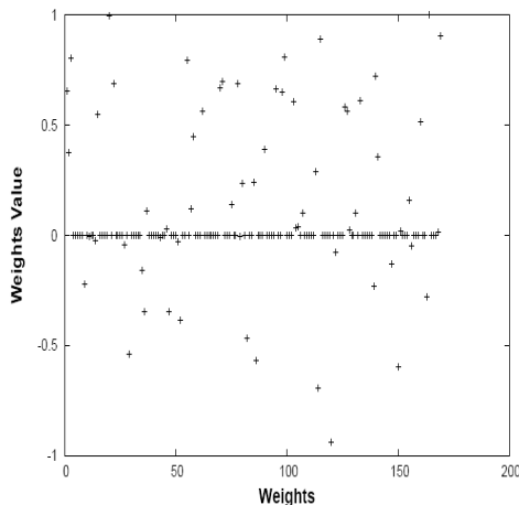
Fig. 12.5(c) Scatter Plot of Weights for a Gene Network
