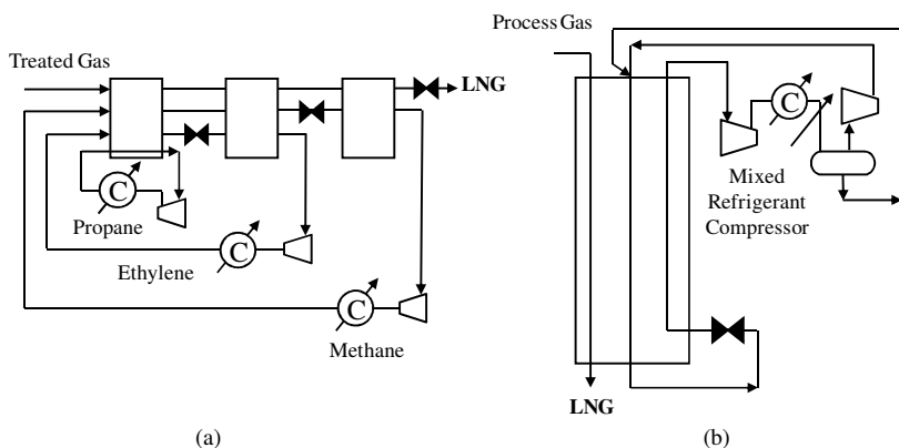
Fig. 8.1 (a) Phillips optimized cascade process for LNG (Houser and Krusen, 1996); (b) PRICO process for LNG (Swenson, 1977). Rectangular boxes are the multi-stream heat exchangers.
