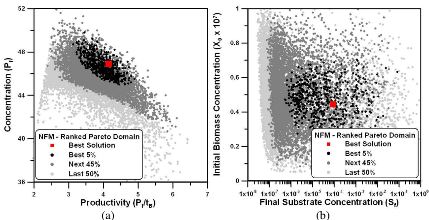
Fig. 7.8 Ranked Pareto domain for the four-objective optimization of gluconic acid using NFM: (a) concentration versus productivity of gluconic acid; (b) Initial inoculum biomass concentration versus final substrate concentration.
