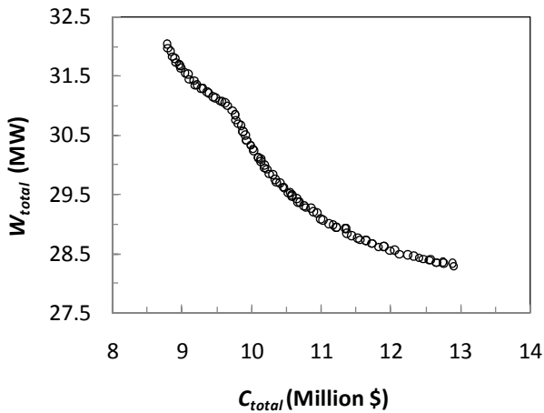
Fig. 8.18 Pareto-optimal front for the optimization of dual independent expander refrigeration process.
