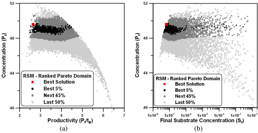
Fig. 7.10 Ranked Pareto domain for the three-objective optimization with RSM using the P and NP rules of Table 7.11: (a) concentration versus productivity of gluconic acid; (b) gluconic acid concentration versus final substrate concentration.
