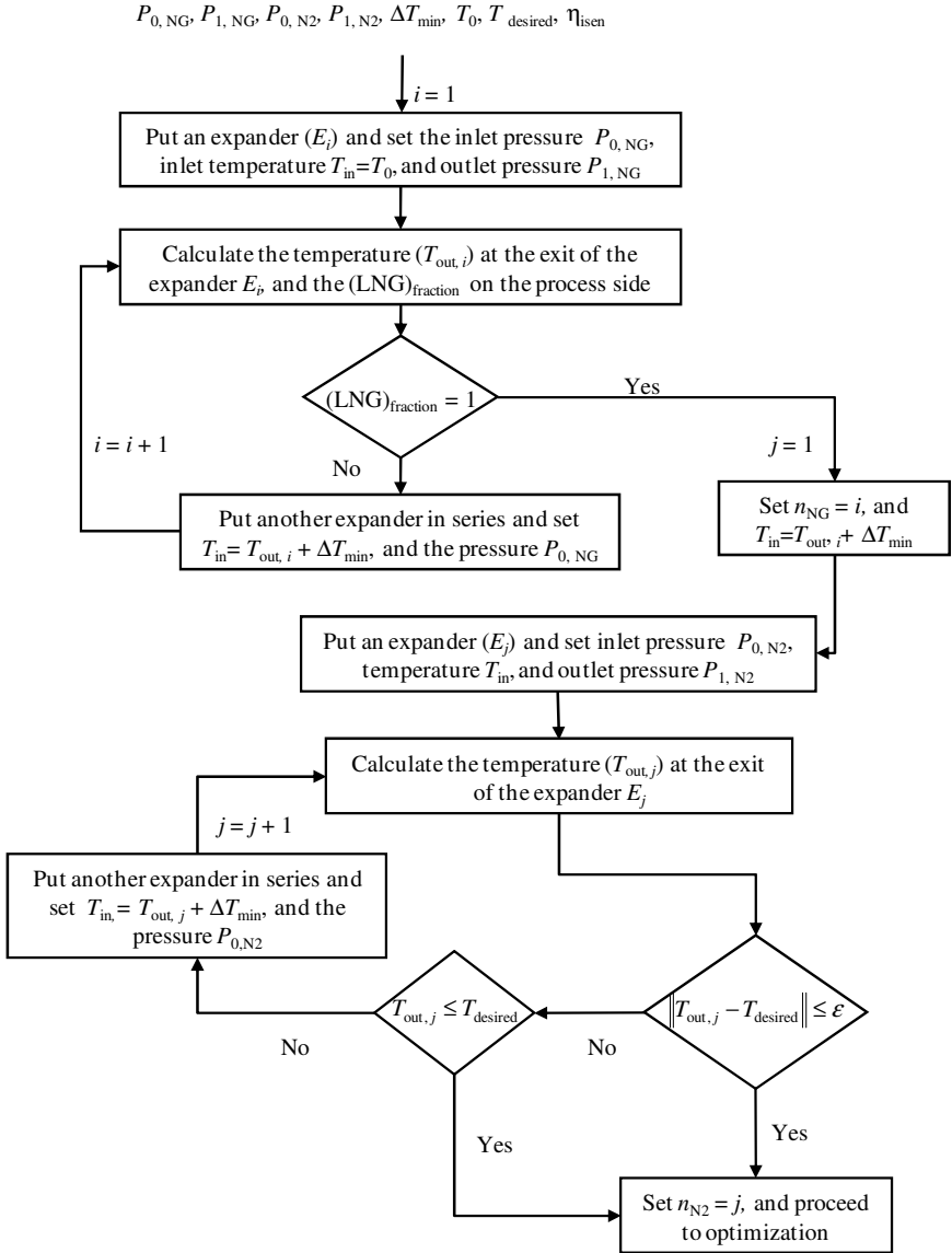
Fig. 8.17 Algorithm to calculate the number of natural gas and number of nitrogen refrigeration stages for the dual independent expander refrigeration process for LNG.
