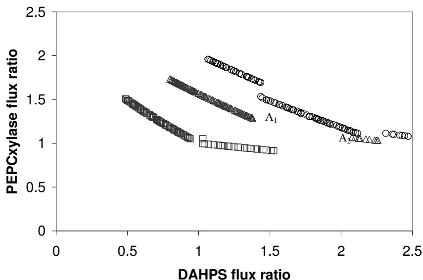
Fig. 13.3A Pareto-optimal fronts for gene manipulations (1-enzyme □; 2-enzyme Δ; 3-enzyme ○) in simultaneous maximization of DAHPS and PEPCxylase flux ratios (Case A).
