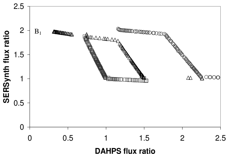
Fig. 13.4A Pareto-optimal fronts for gene manipulations (1-enzyme \square ; 2-enzyme \Delta ; 3-enzyme \circ ) in simultaneous maximization of DAHPS and SerSynth flux ratios (Case B).
