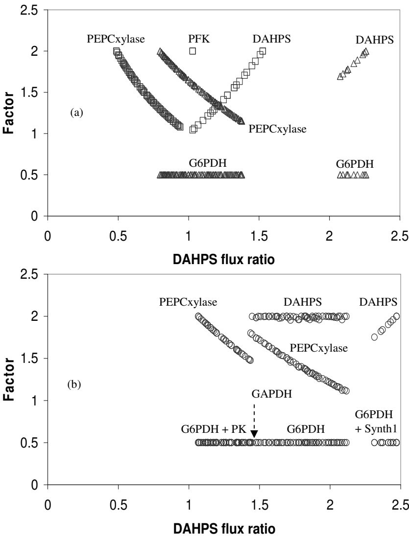
Fig. 13.3B Pareto-optimal enzyme manipulation factors in simultaneous maximization of DAHPS and PEPCxylase flux ratios (Case A) (a) 1-enzyme ( \square ) and 2-enzyme ( \Delta ) manipulation factor and (b) 3-enzyme manipulation factor ( \circ ).
