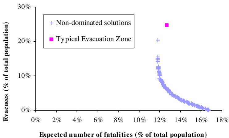
Fig. 11.6 Non-dominated solutions (ERPs) in case of a BLEVE phenomenon in an LPG storage tank (“capacity” of the transportation network: 1, “warning time”: 1800 sec).
