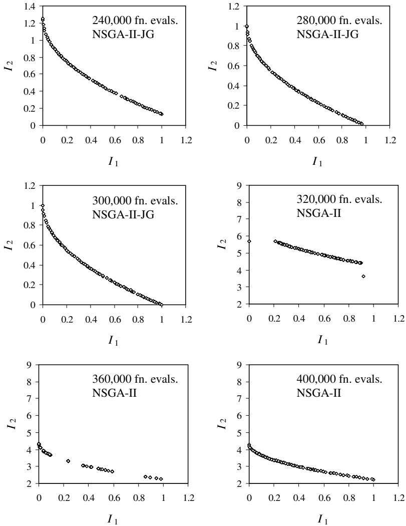
Fig. 4.12 Plots of non-dominated solutions obtained with NSGA-II-JG after 240,000 – 300,000 function evaluations (fn. evals.) and for NSGA-II for 320,000 – 400,000 fn. evals. for the ZDT4 problem. Note that I_1 and I_2 extend over [0, 1] (global Pareto set) for NSGA-II-JG only after about 300,000 function evaluations, and do not show this characteristic for NSGA-II
