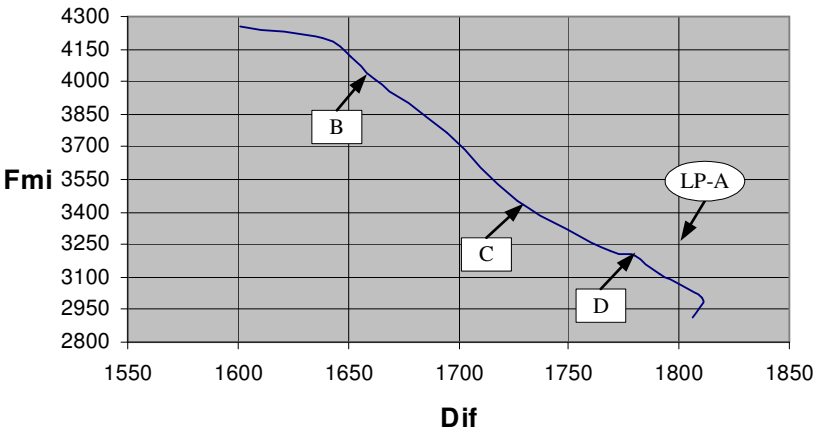
Fig. 9.6 Conflicting objectives: Fmi Versus Dif .
