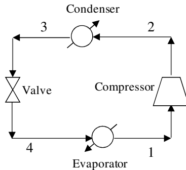
Fig. 8.2 A simple compression refrigeration cycle.
