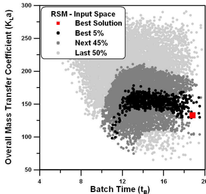
Fig. 7.11 Plot of the input space for the three-objective Pareto domain using RSM: K_La versus t_B .
