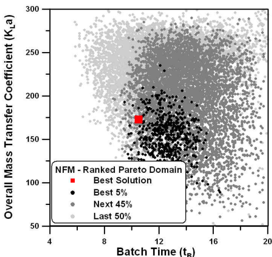
Fig. 7.17 Plot of the input space for the four-objective Pareto domain using RSM with relative weights: K_{La} versus t_B .
