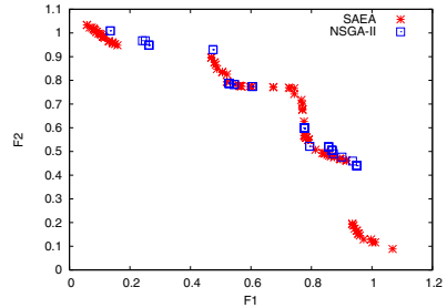
Fig. 5.6 Results of TNK obtained by SAEA and NSGA-II using the same number of function evaluations
