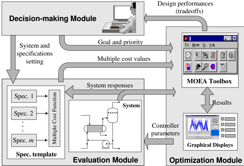
Fig. 9.2 The evolutionary optimization architecture.
