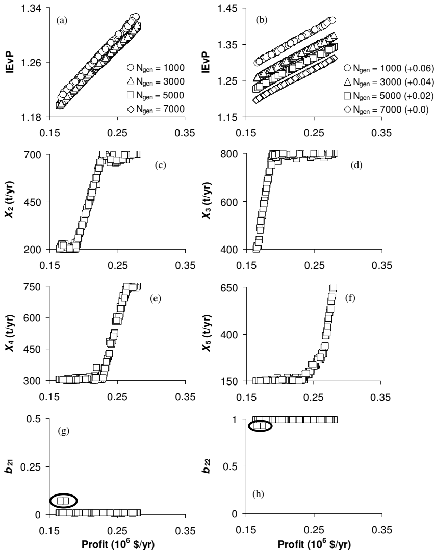
Fig. 10.9 MOO of the IE with 6 plants for maximizing profit and minimizing IEvP; for clarity, results in (a) are re-plotted in (b) with suitable vertical shifts; Profit is shown on the x-axis in all plots.
