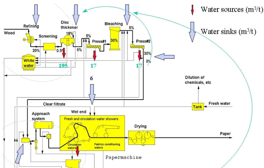
Fig. 6.4. Water sinks and sources in an integrated plant. (This figure is available in color in the file water_allocation.jpg in Chapter 6 on the CD.)
