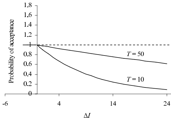
Fig. 4.8 Probability of acceptance of any solution in SSA
