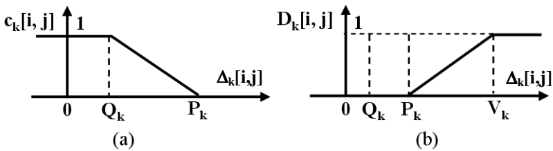
Fig. 7.2 (a) Individual concordance index, and (b) discordance index calculations used in NFM algorithm to determine ranking scores for the Pareto domain solutions.
